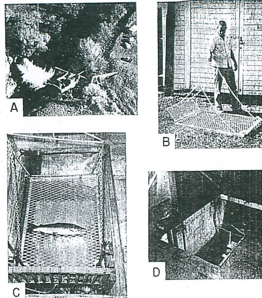
FIGURE 9. Mill Creek Counting Station. A, aerial view of Clough Dam, showing a fishway and house trailer which is used as a residence by the fish counter; B, elevator type bottom used in trap, so that captured fish could be raised for better viewing; C, trap in use, showing how steelhead were raised to examine them for marks and tags; D, the trap in fishing position in the fishway. Photographs by John E. Rigg.
